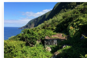
Fajã de Manuel Teixeira Fajã de Manuel Teixeira (cliff)
